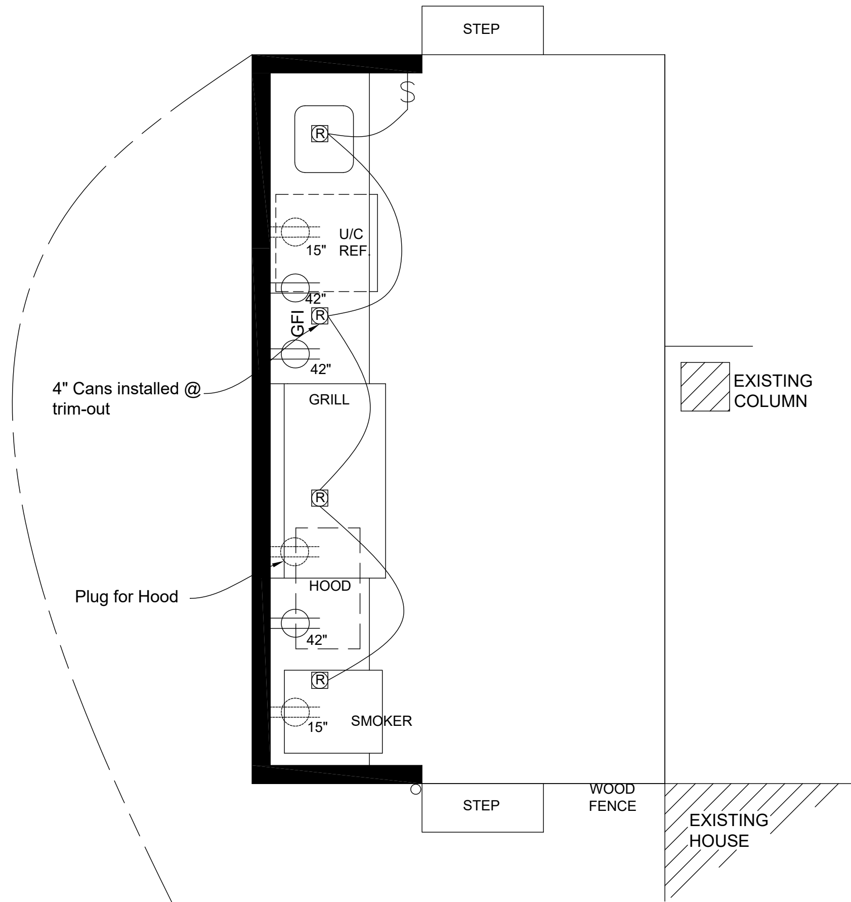
1 2 ELECTRICAL PLAN SCALE : 1/2"=1'-0"
