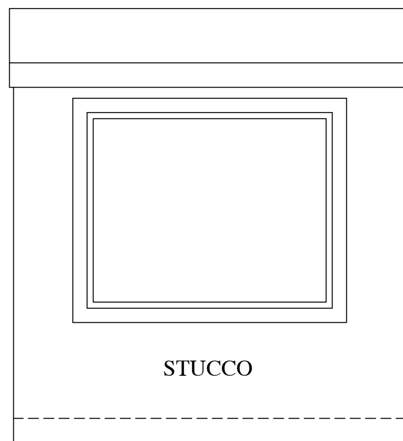
4 5 FRONT ELEVATION
