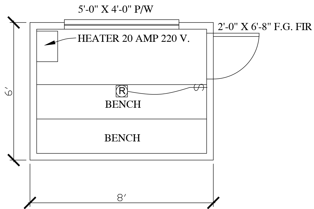
1 5 FLOOR PLAN
